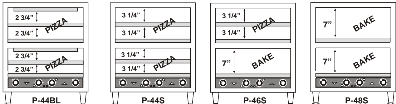
Figure C DECK ARRANGEMENT BY MODEL
