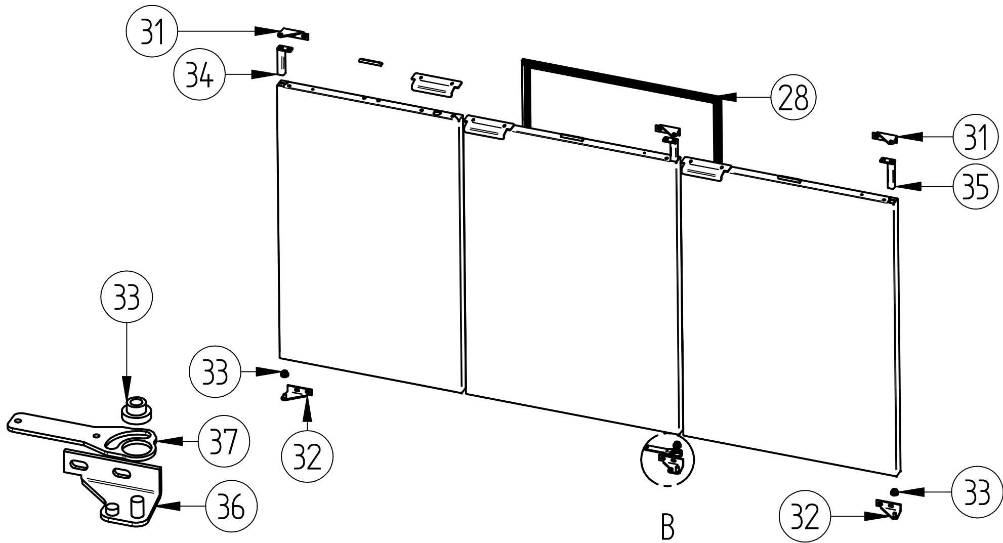
DETAIL B
